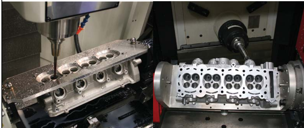
Multiple 5 Axis CNC Head Porting Machines
